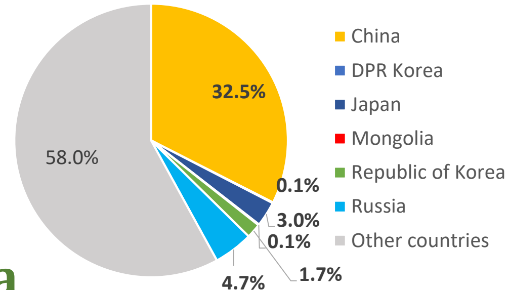
Global CO 2 Emissions from Fossil Fuels (Data: EDGAR, European Commission 2020)
